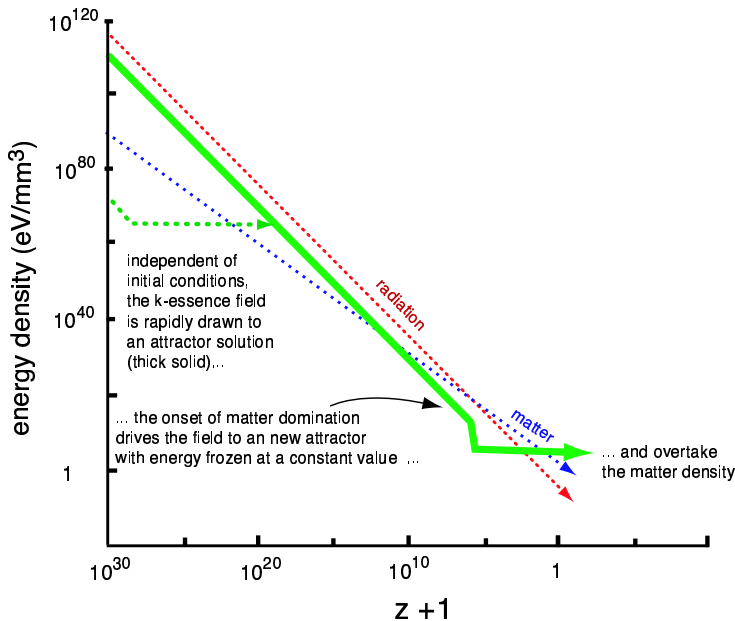
FIG. 1. A plot showing the matter, radiation, and quintessence energy density as a function of red shift for the case of k -essence models. The k -essence models are special cases of “tracker” models with dynamical attractor solutions that funnel a wide range of initial conditions into a common evolutionary track (upper left). The distinctive property of k -essence is that the behavior shifts at the onset of matter domination to an attractor solution that acts like a cosmological constant (bottom). The bars below the graph indicate important events in cosmic history. The late conversion to a cosmological constant behavior explains why cosmic acceleration has begun only recently, a modest period (in terms of temperature scale) after matter domination.
