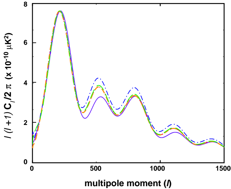
FIG. 8. Comparison of higher multipole moments of the CMB temperature power spectrum for the models in Fig. 7. The spectra have been normalized so that the amplitudes match at the top of the first acoustic peak.
