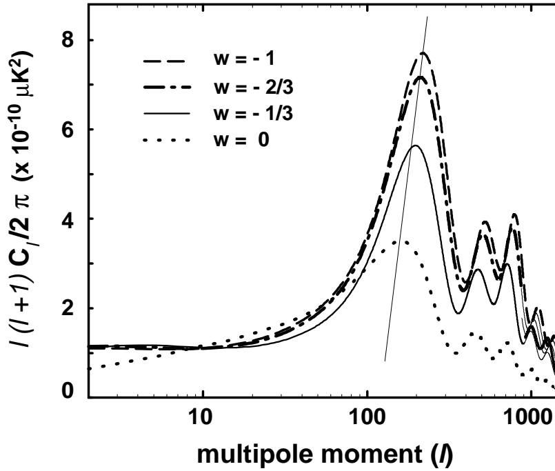
FIG. 2. The cosmic microwave background power spectrum (multipole moments C_\ell vs. multipole number \ell ) for a sequence of models with identical parameters except for varying w . Note the small shift in the position of the first acoustic peak, as indicated by the tilted line.
