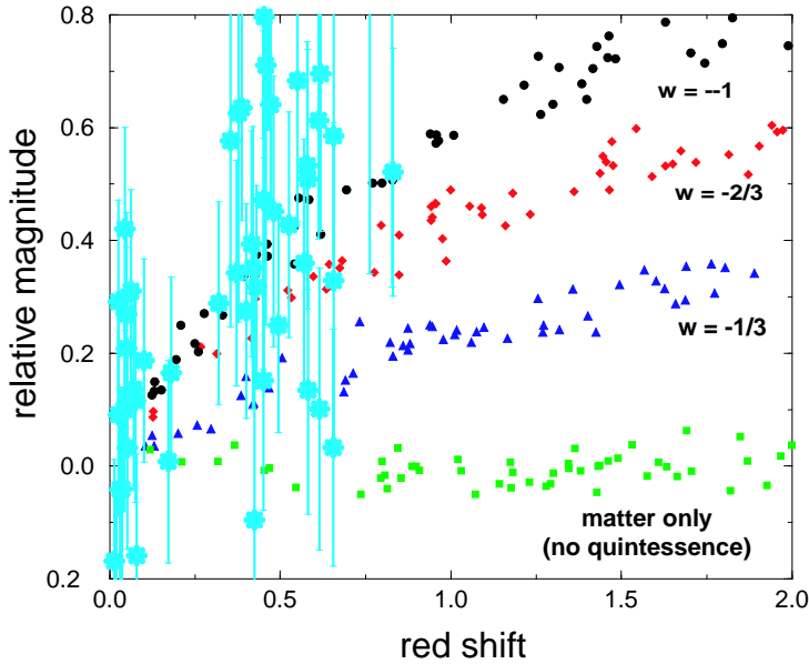
FIG. 4. Magnitude versus red shift relative to a model with no quintessence ( \Omega_m = 1 ) for \Omega_m = 0.3 and w = -1, -2/3, -1/3 and 0. Small symbols represent the optimal that can be achieved by measuring thousands of supernovae and binning by red shift. Data point with error bars (on left) represent current data from individual galaxies.
